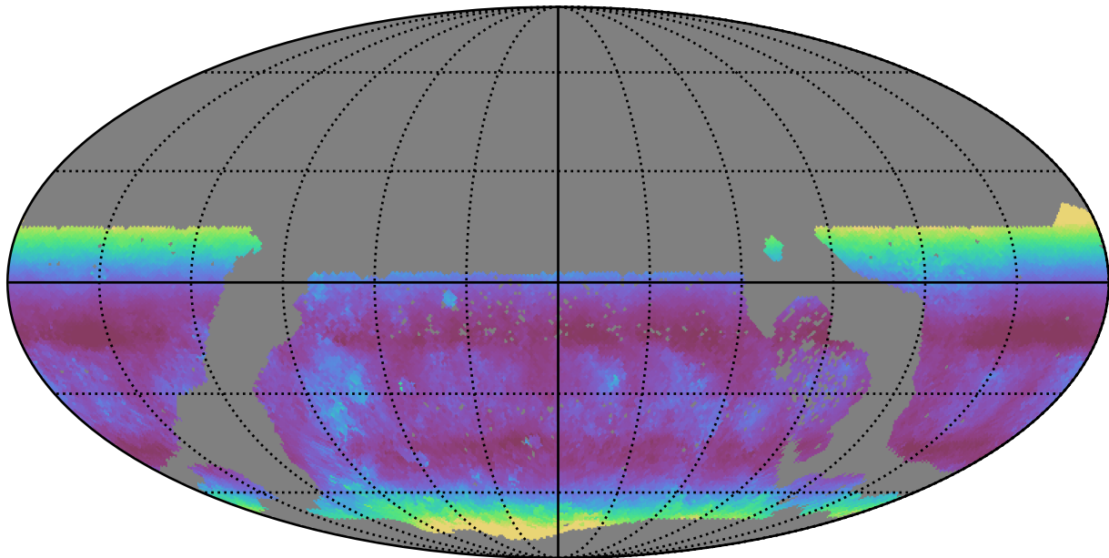
too_elab_r8_d2_giz_v3.4_10yrs WFD g band: Median airmass
