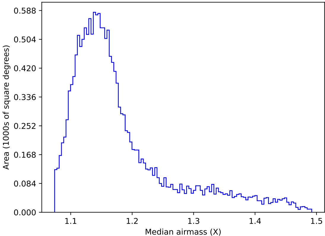
too_elab_r8_d2_giz_v3.4_10yrs WFD g band: Median airmass
