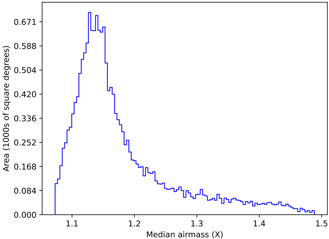
too_elab_r8_d2_giz_v3.4_10yrs WFD g band: Median airmass
