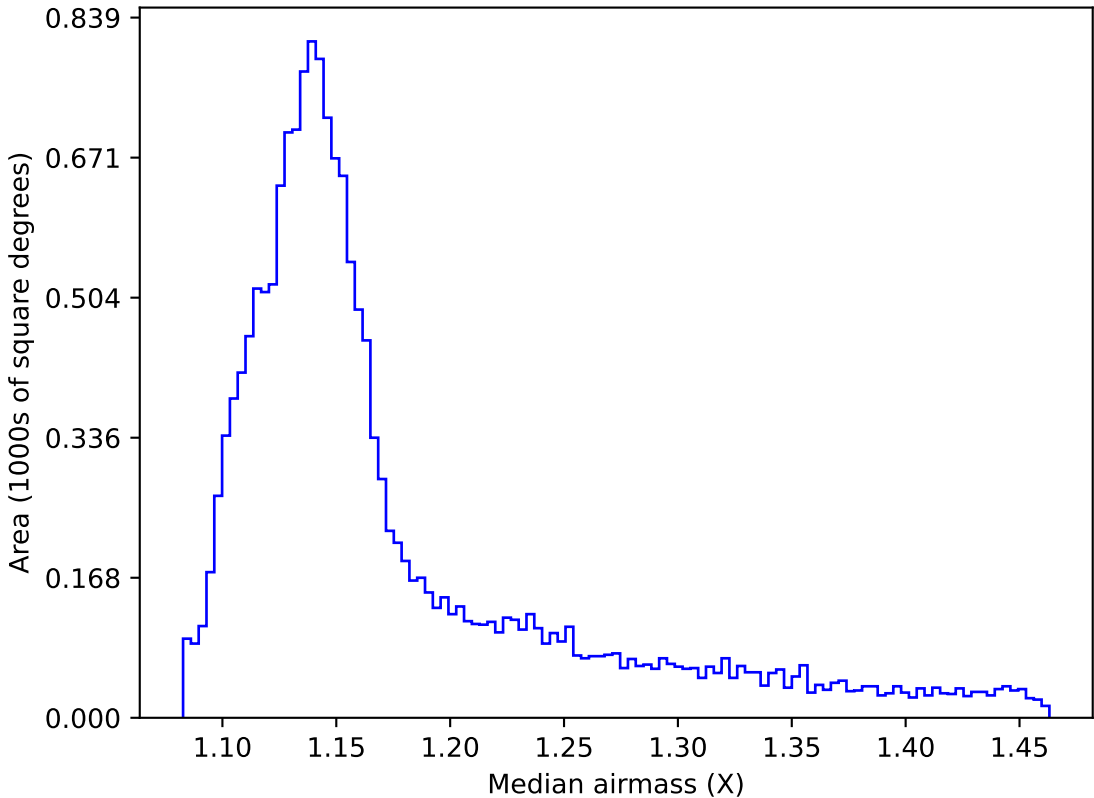
too_elab_r8_d2_giz_v3.4_10yrs WFD all bands: Median airmass
