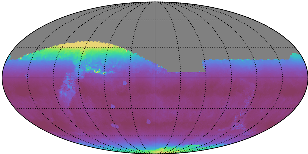
too_elab_r8_d2_giz_v3.4_10yrs All sky z band: Median airmass
