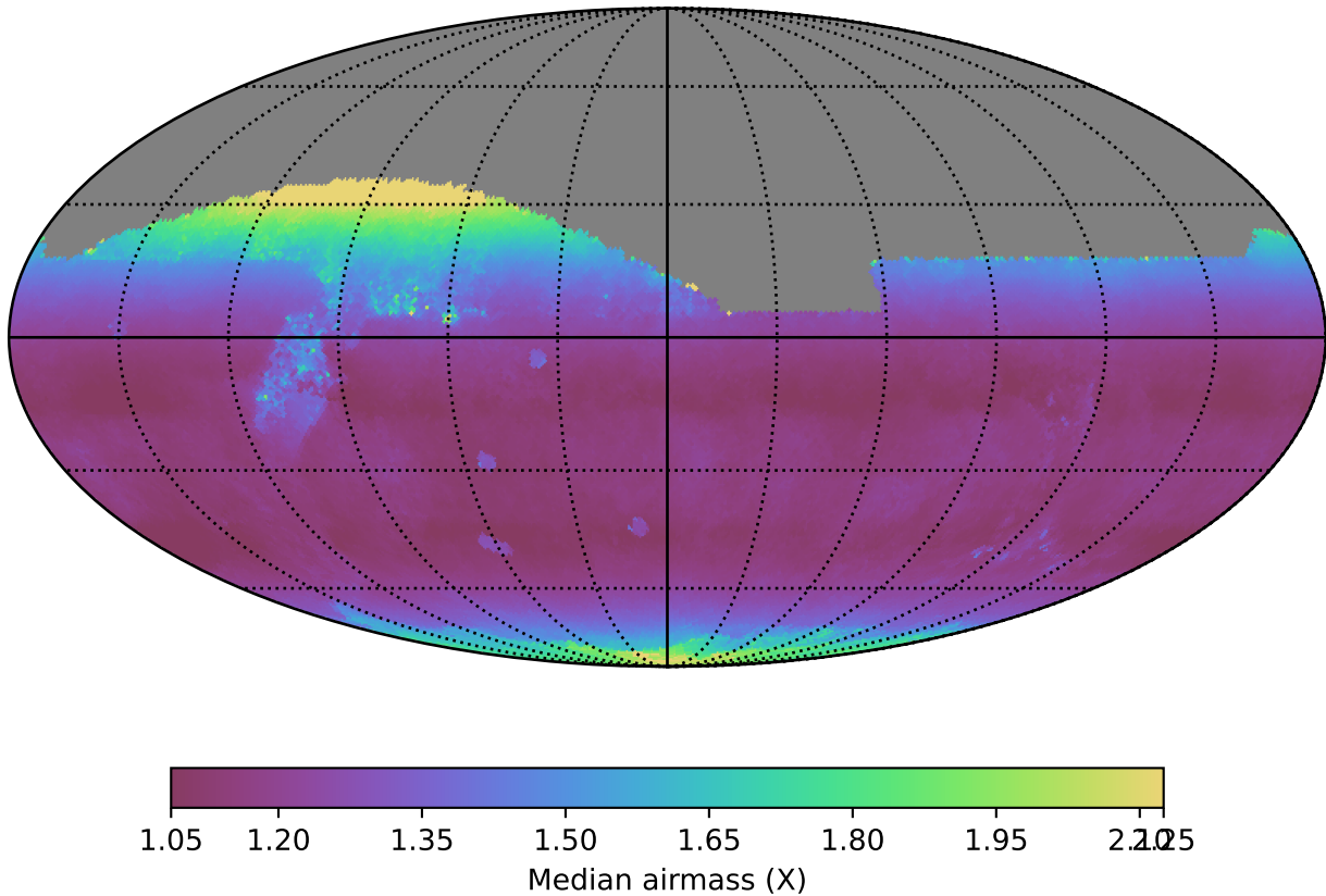
too_elab_r8_d2_giz_v3.4_10yrs All sky z band: Median airmass
