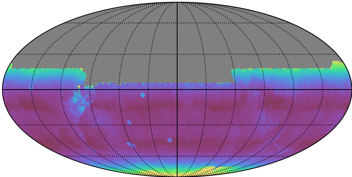
too_elab_r8_d2_giz_v3.4_10yrs All sky y band: Median airmass
