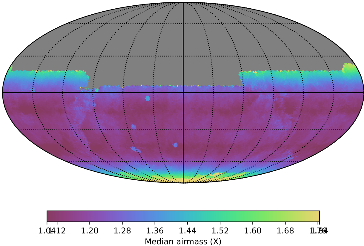
too_elab_r8_d2_giz_v3.4_10yrs All sky y band: Median airmass
