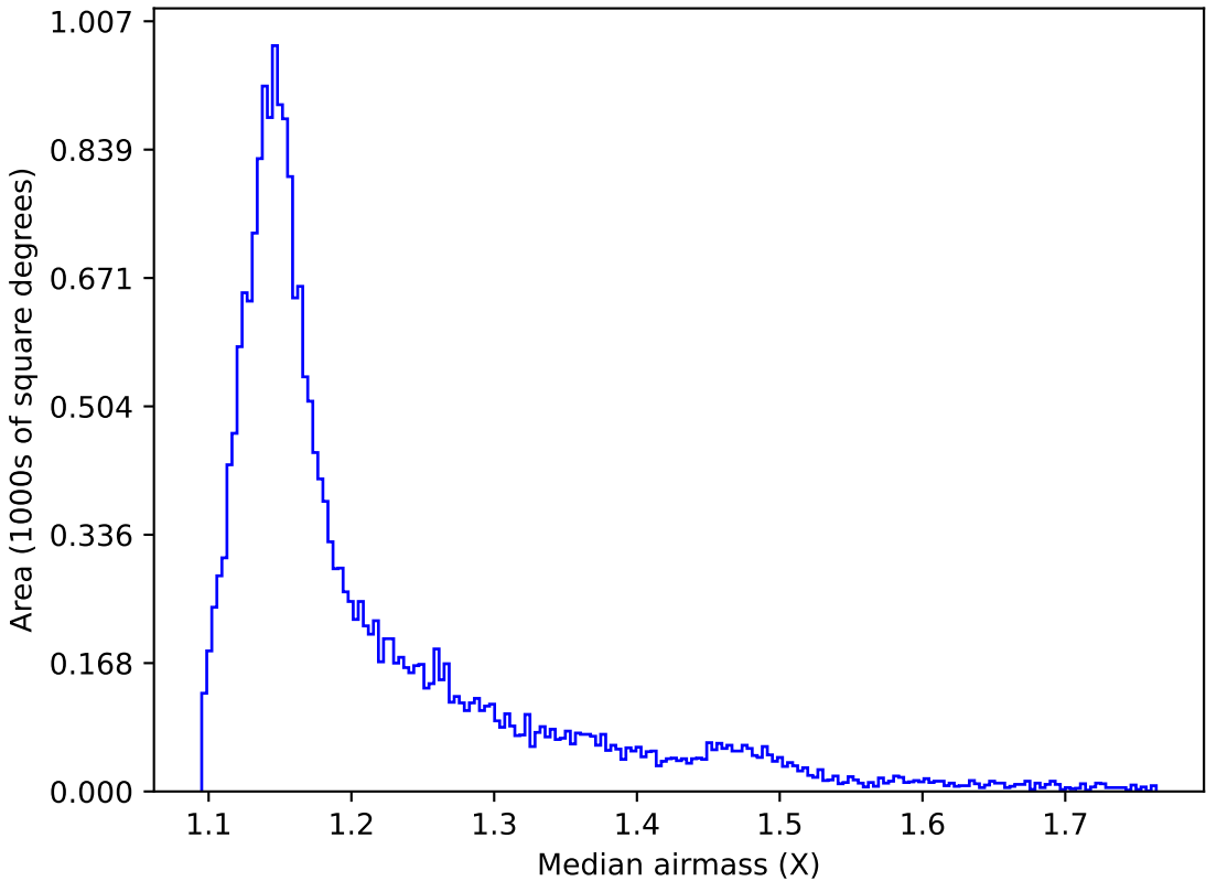
too_elab_r8_d2_giz_v3.4_10yrs All sky y band: Median airmass
