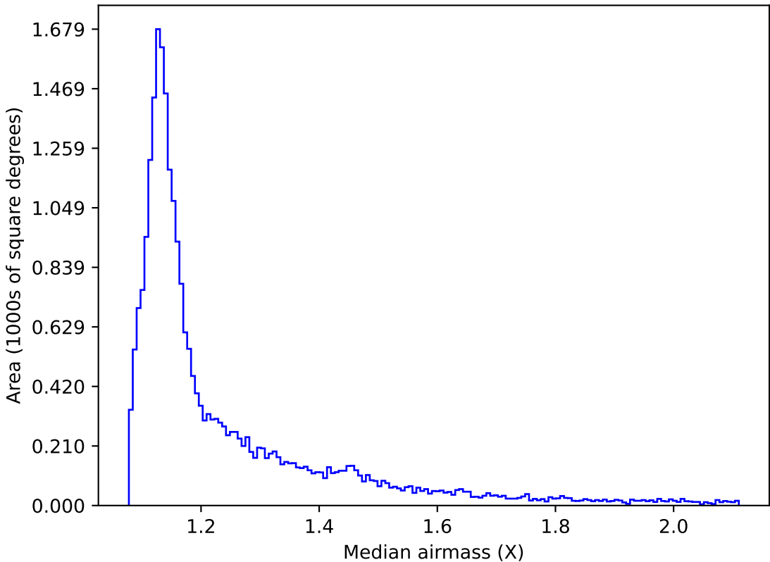
too_elab_r8_d2_giz_v3.4_10yrs All sky r band: Median airmass
