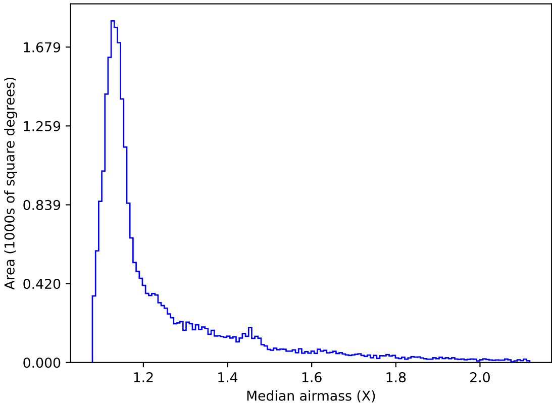
too_elab_r8_d2_giz_v3.4_10yrs All sky i band: Median airmass
