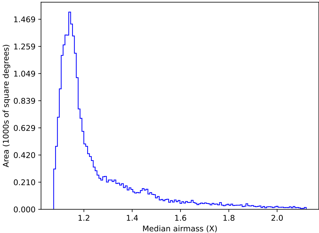
too_elab_r8_d2_giz_v3.4_10yrs All sky g band: Median airmass
