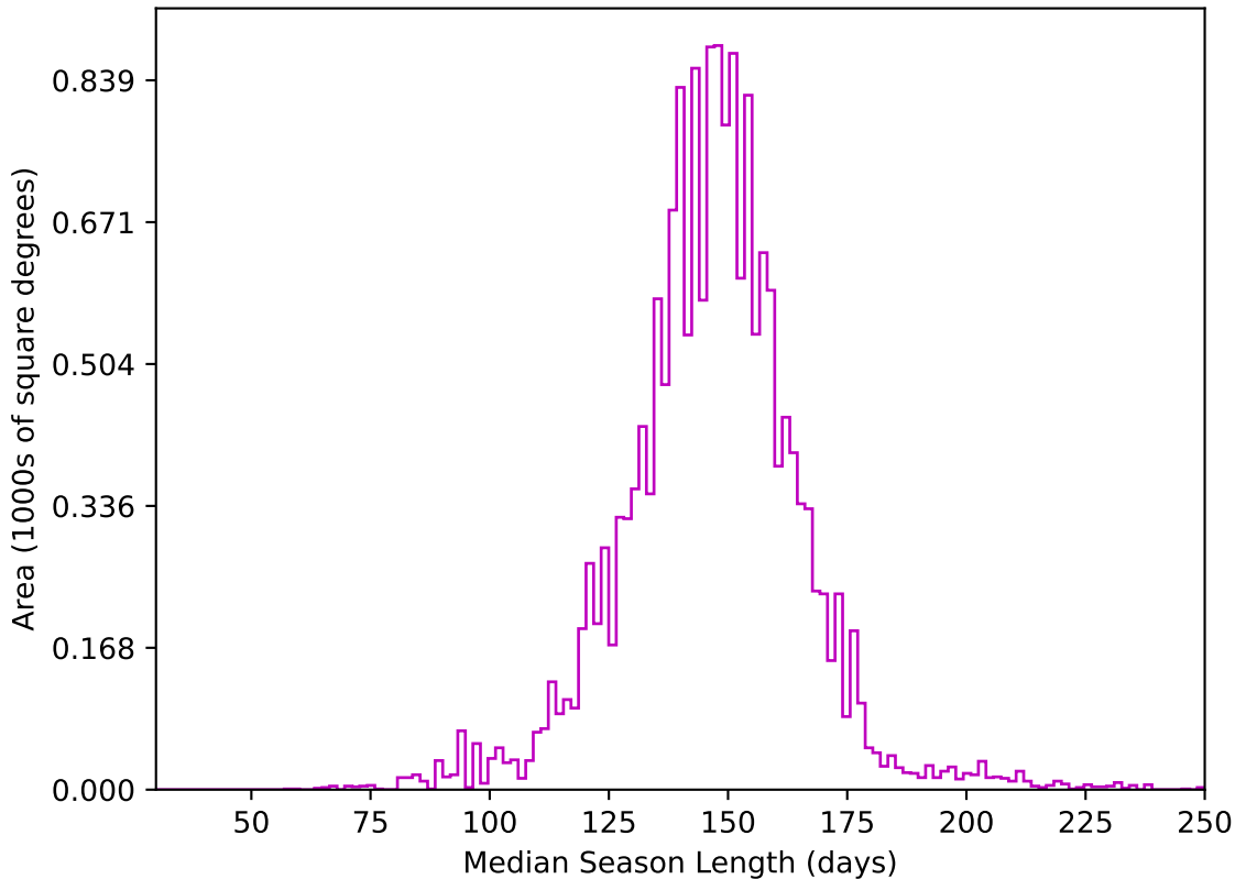
too_elab_r8_d2_giz_v3.4_10yrs WFD z band: Median Season Length
