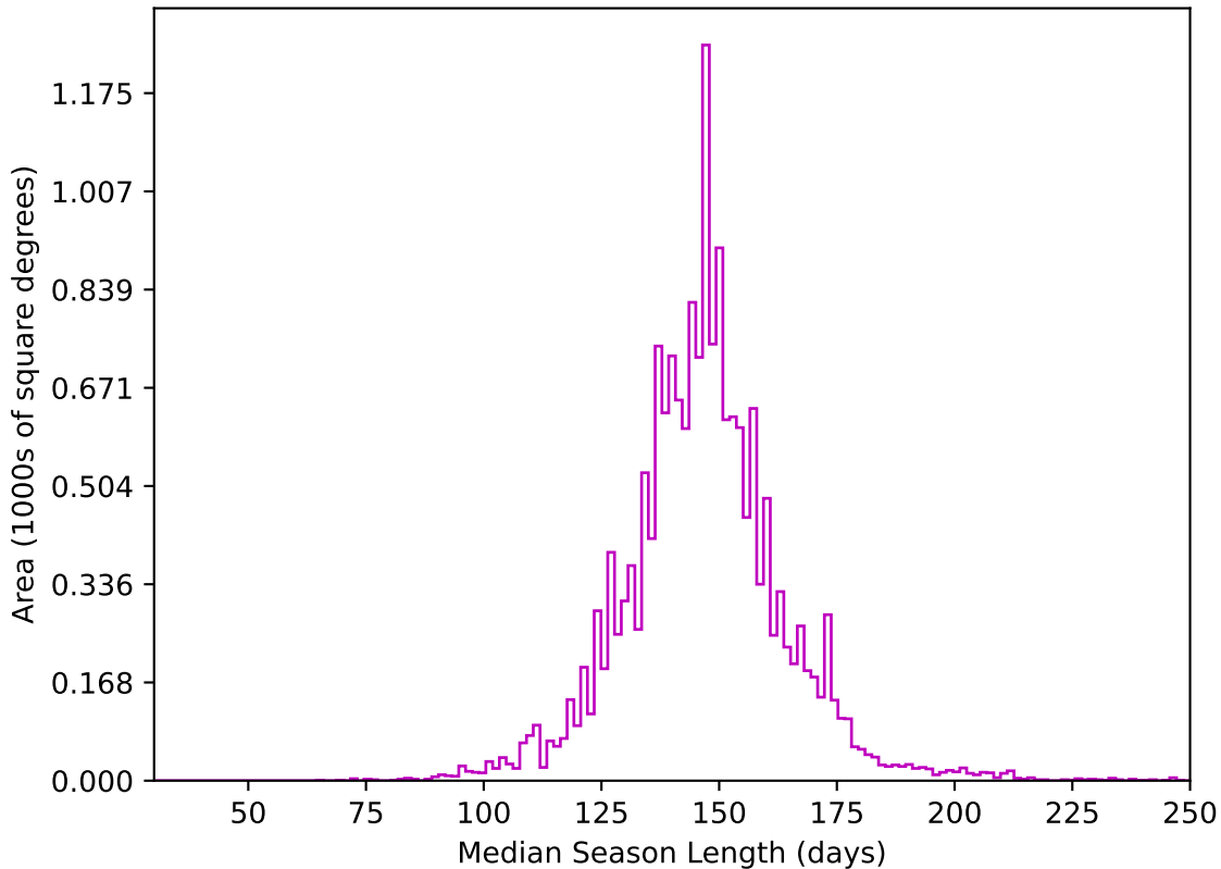
too_elab_r8_d2_giz_v3.4_10yrs WFD z band: Median Season Length
