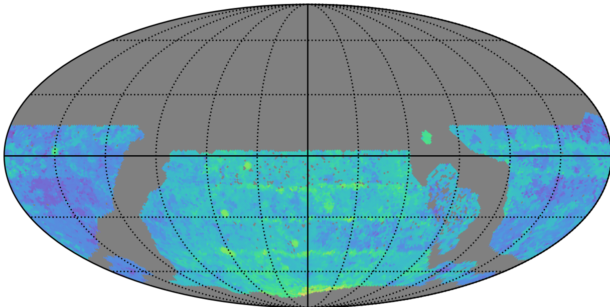
too_elab_r8_d2_giz_v3.4_10yrs WFD y band: Median Season Length
