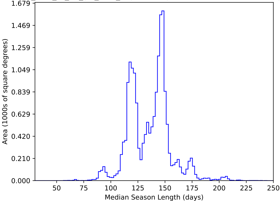
too_elab_r8_d2_giz_v3.4_10yrs WFD y band: Median Season Length
