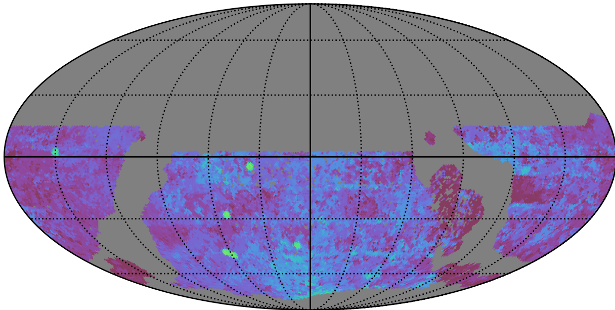
too_elab_r8_d2_giz_v3.4_10yrs WFD u band: Median Season Length
