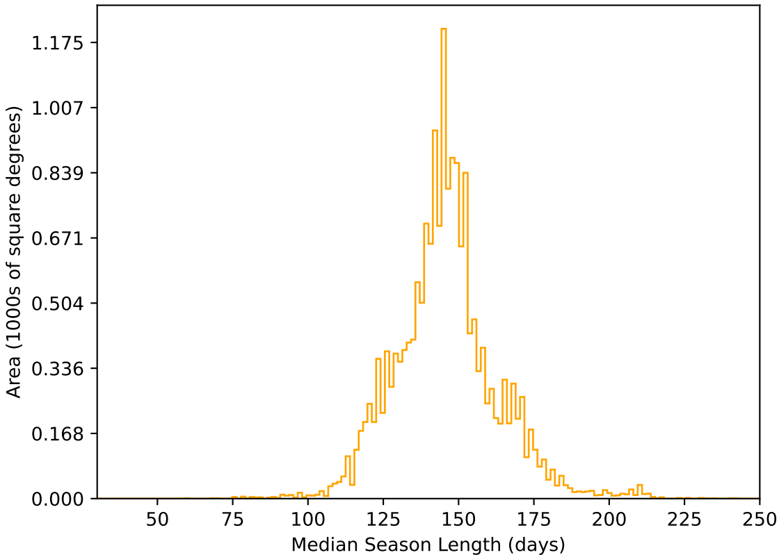
too_elab_r8_d2_giz_v3.4_10yrs WFD r band: Median Season Length
