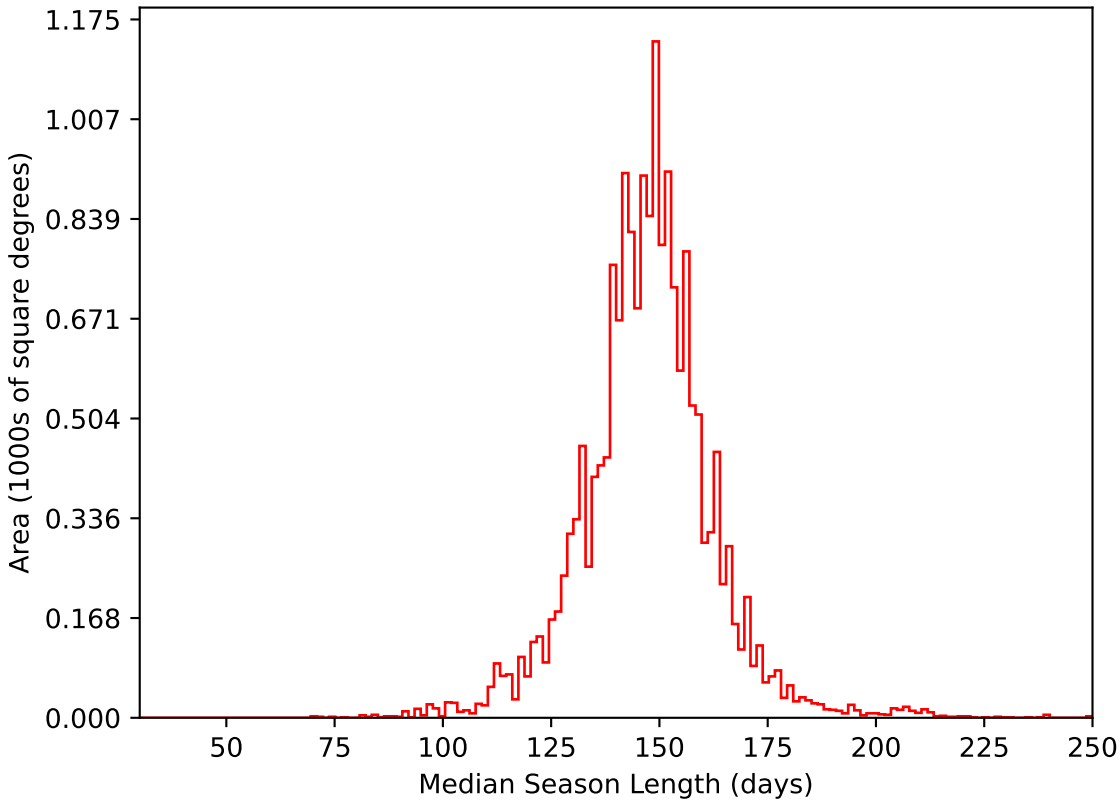
too_elab_r8_d2_giz_v3.4_10yrs WFD i band: Median Season Length
