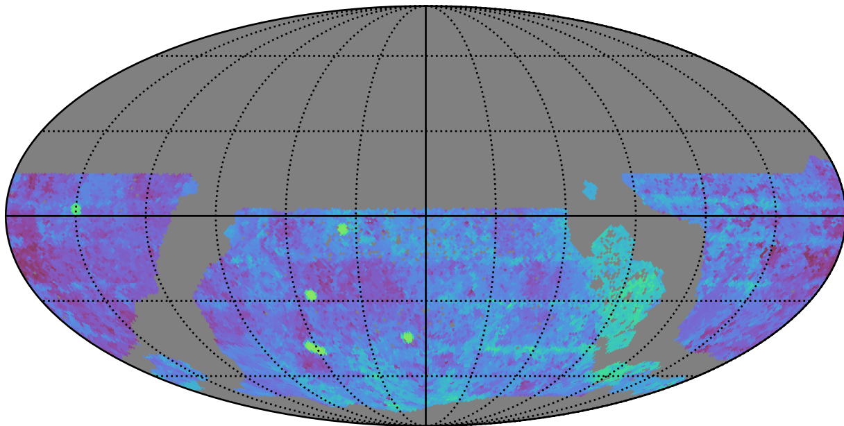
too_elab_r8_d2_giz_v3.4_10yrs WFD g band: Median Season Length
