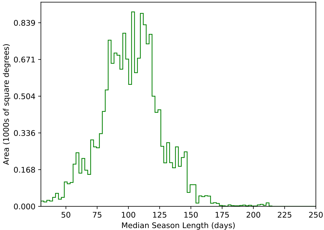
too_elab_r8_d2_giz_v3.4_10yrs WFD g band: Median Season Length
