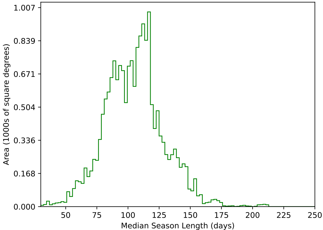
too_elab_r8_d2_giz_v3.4_10yrs WFD g band: Median Season Length
