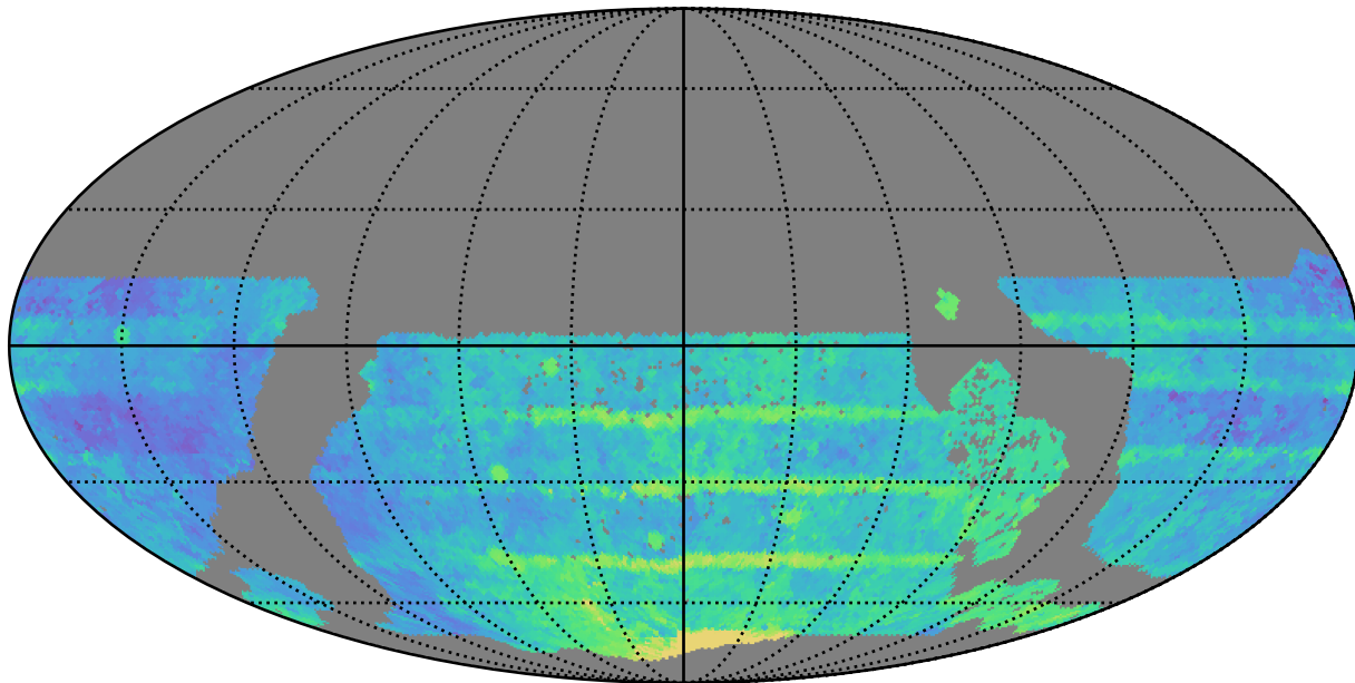
too_elab_r8_d2_giz_v3.4_10yrs WFD all bands: Median Season Length
