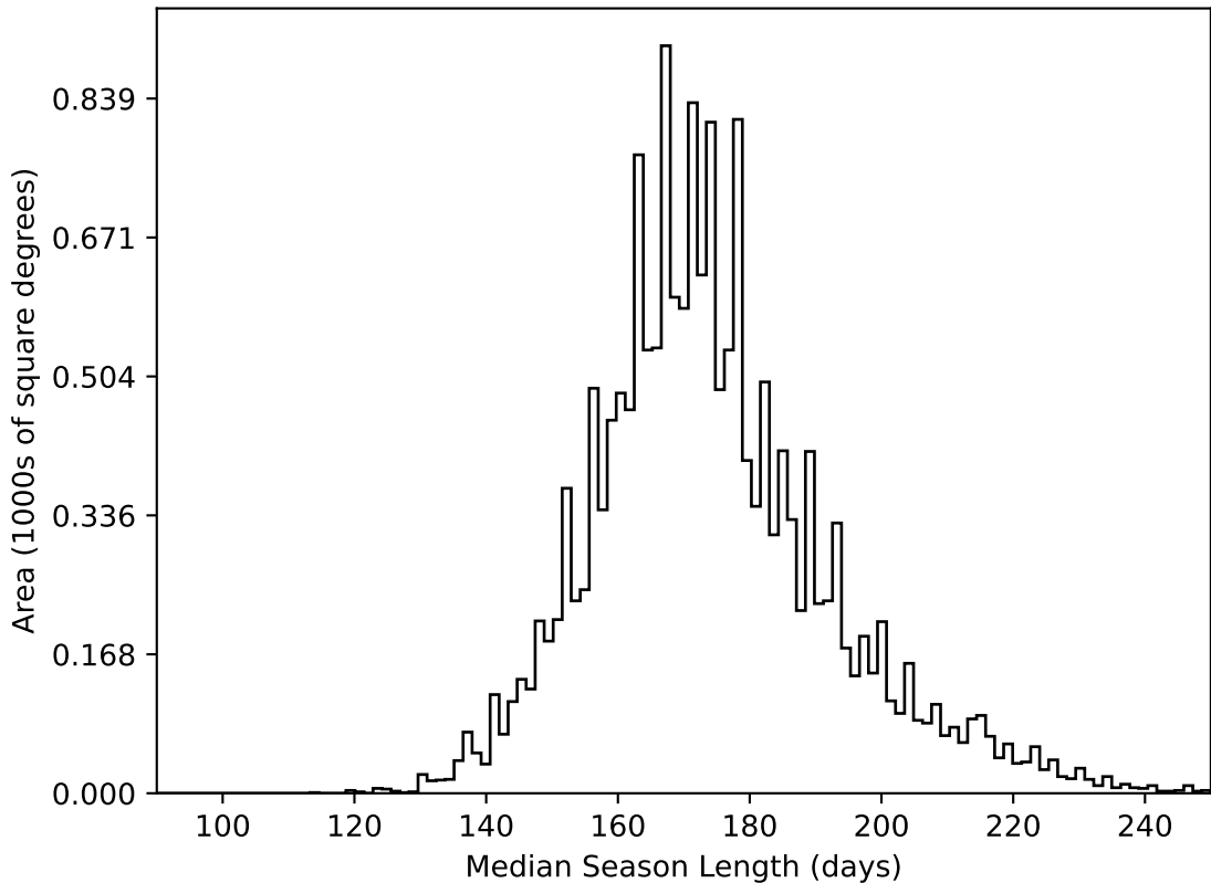
too_elab_r8_d2_giz_v3.4_10yrs WFD all bands: Median Season Length
