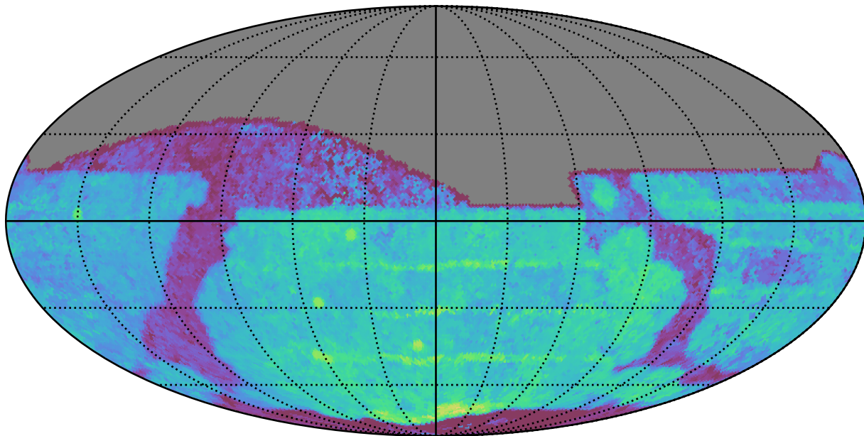
too_elab_r8_d2_giz_v3.4_10yrs All sky z band: Median Season Length
