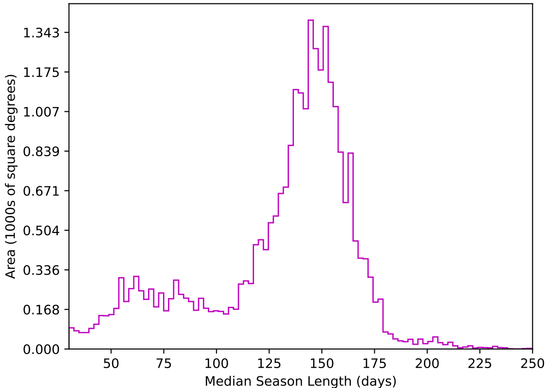
too_elab_r8_d2_giz_v3.4_10yrs All sky z band: Median Season Length
