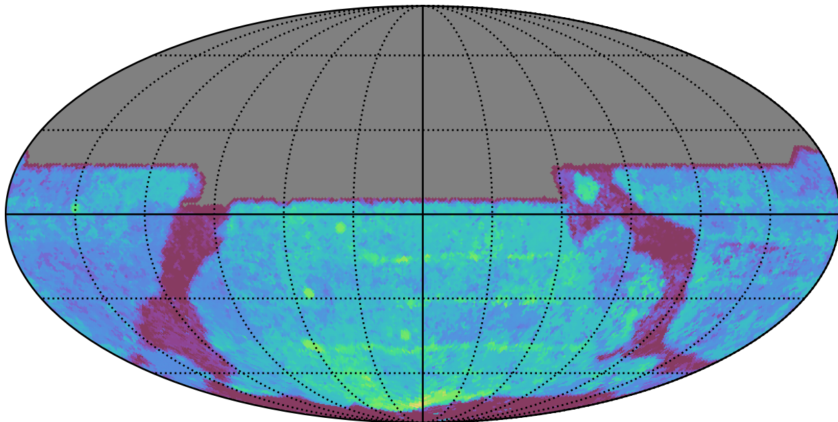
too_elab_r8_d2_giz_v3.4_10yrs All sky y band: Median Season Length
