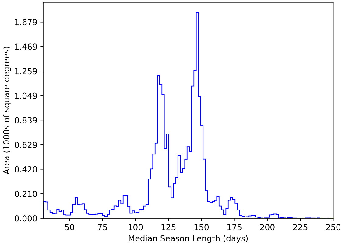
too_elab_r8_d2_giz_v3.4_10yrs All sky y band: Median Season Length
