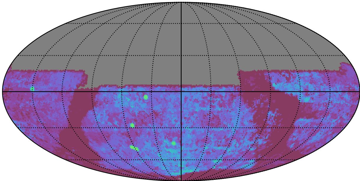
too_elab_r8_d2_giz_v3.4_10yrs All sky u band: Median Season Length
