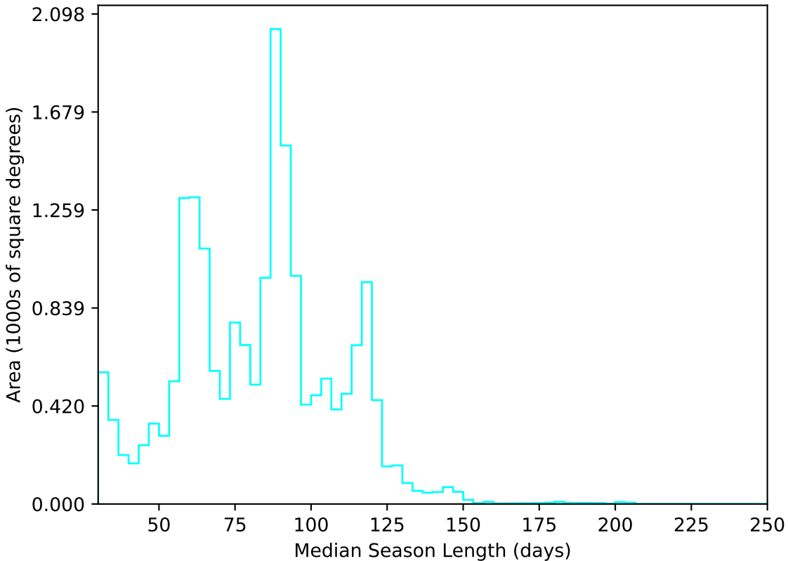
too_elab_r8_d2_giz_v3.4_10yrs All sky u band: Median Season Length
