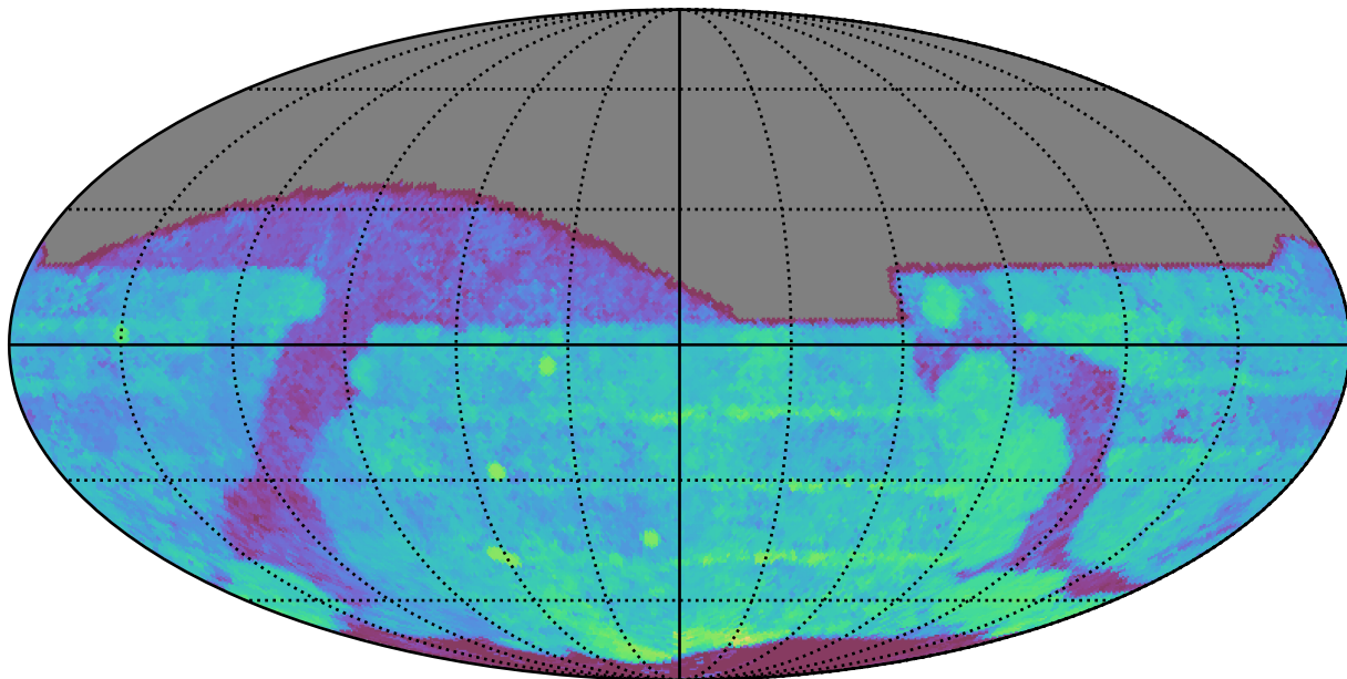
too_elab_r8_d2_giz_v3.4_10yrs All sky r band: Median Season Length
