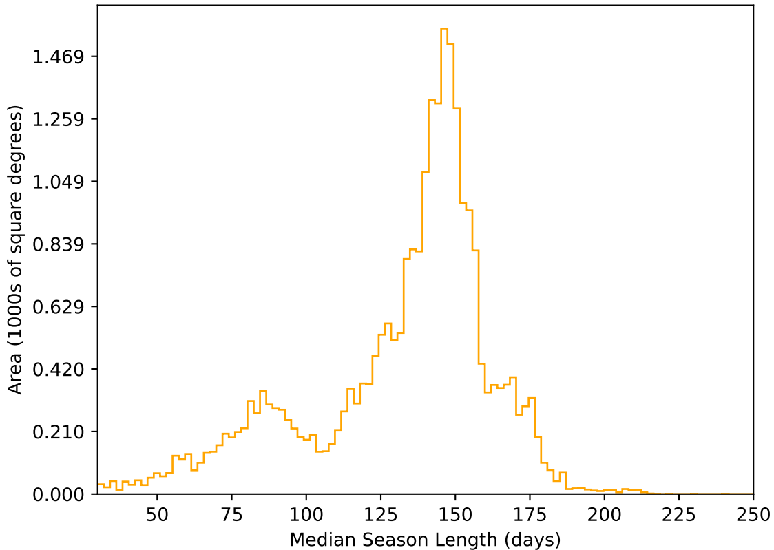
too_elab_r8_d2_giz_v3.4_10yrs All sky r band: Median Season Length
