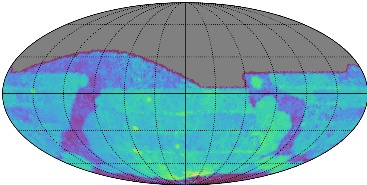
too_elab_r8_d2_giz_v3.4_10yrs All sky i band: Median Season Length
