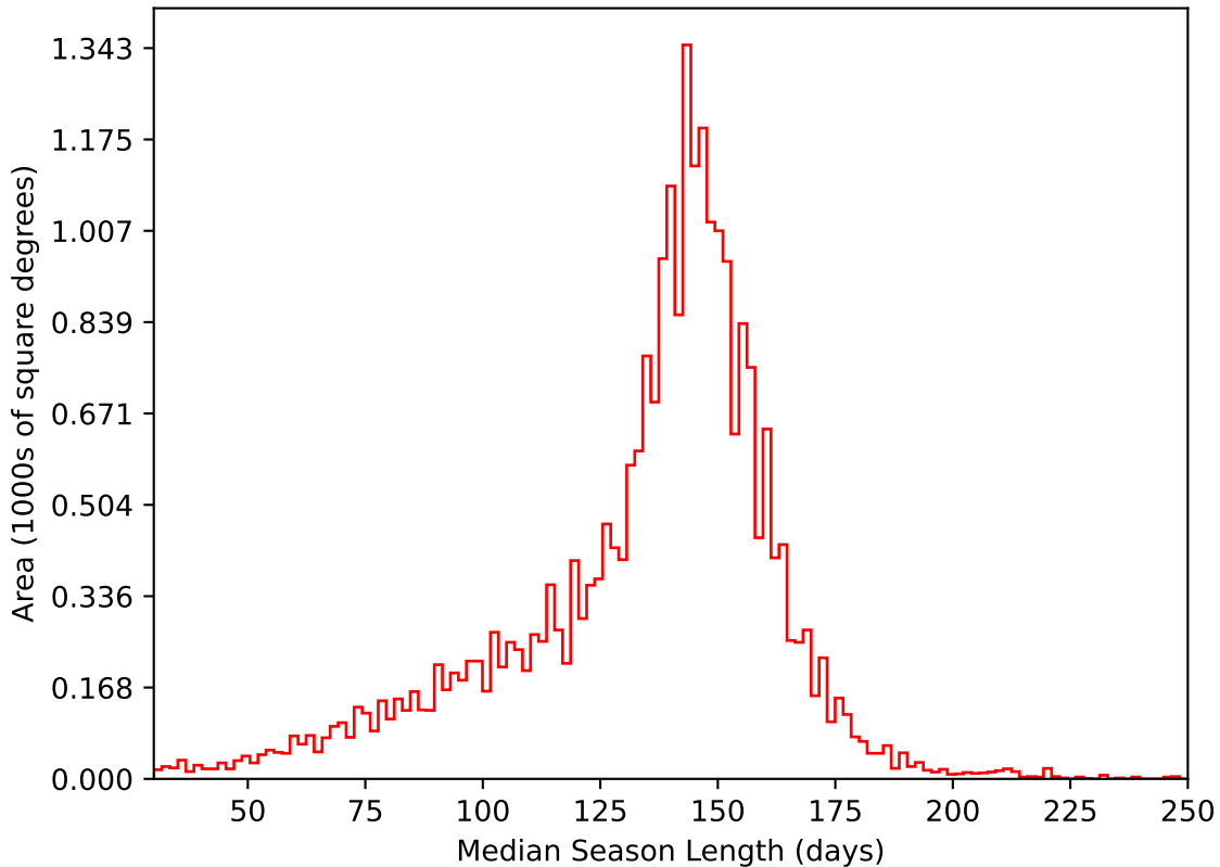
too_elab_r8_d2_giz_v3.4_10yrs All sky i band: Median Season Length
