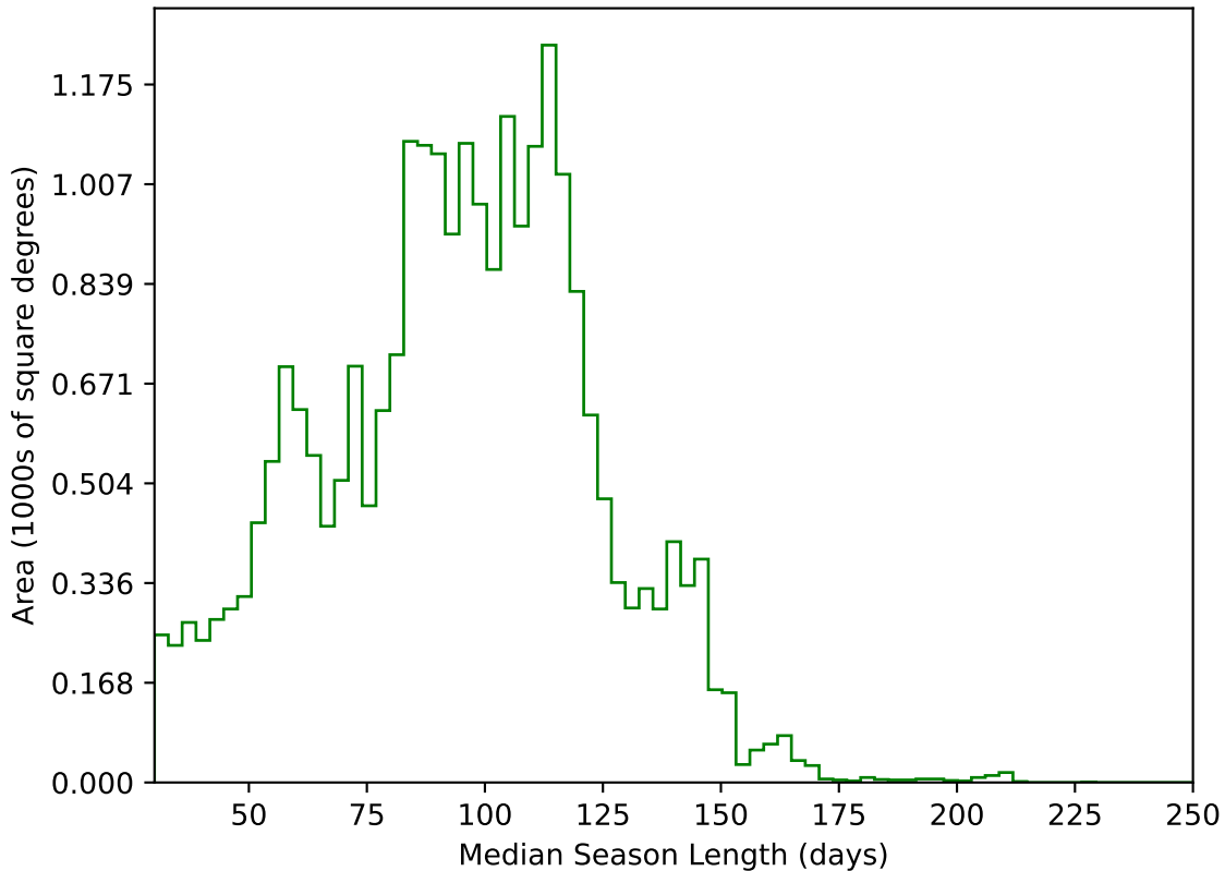
too_elab_r8_d2_giz_v3.4_10yrs All sky g band: Median Season Length
