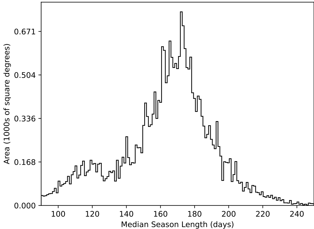
too_elab_r8_d2_giz_v3.4_10yrs All sky all bands: Median Season Length
