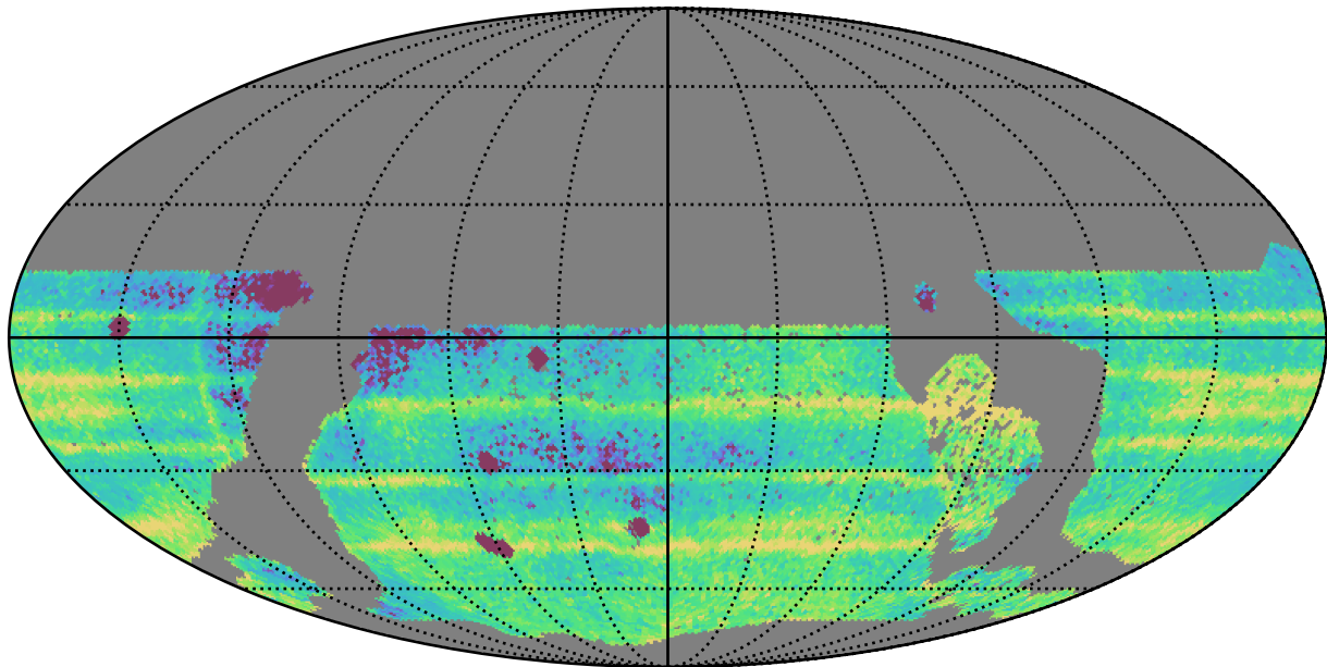
too_elab_r8_d2_giz_v3.4_10yrs WFD: Median Intra-Night Gap
