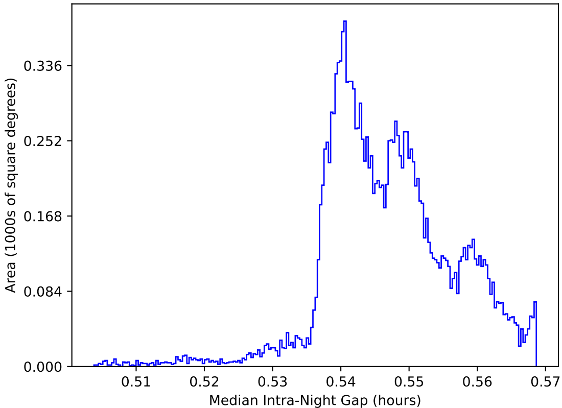
too_elab_r8_d2_giz_v3.4_10yrs WFD: Median Intra-Night Gap
