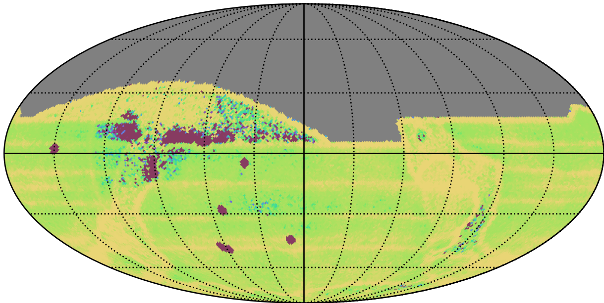
too_elab_r8_d2_giz_v3.4_10yrs All sky: Median Intra-Night Gap
