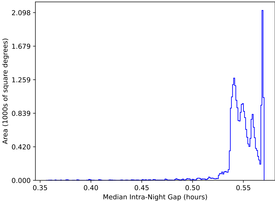
too_elab_r8_d2_giz_v3.4_10yrs All sky: Median Intra-Night Gap
