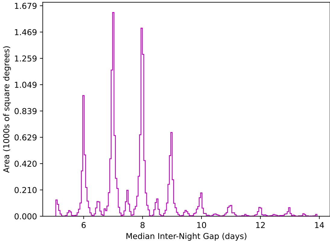
too_elab_r8_d2_giz_v3.4_10yrs WFD z band: Median Inter-Night Gap
