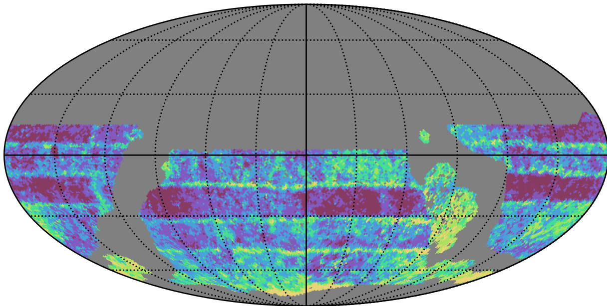
too_elab_r8_d2_giz_v3.4_10yrs WFD r band: Median Inter-Night Gap
