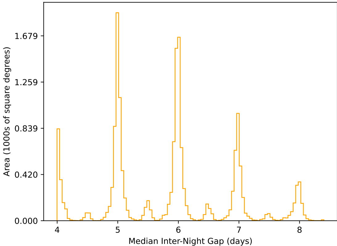
too_elab_r8_d2_giz_v3.4_10yrs WFD r band: Median Inter-Night Gap
