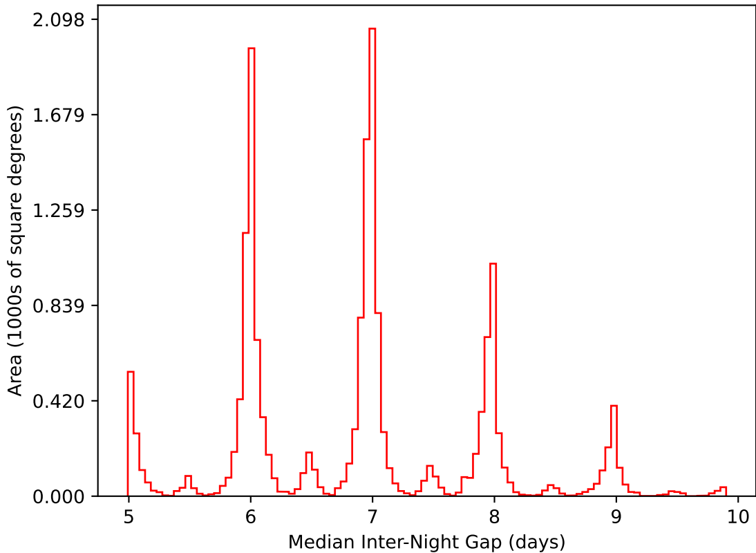
too_elab_r8_d2_giz_v3.4_10yrs WFD i band: Median Inter-Night Gap
