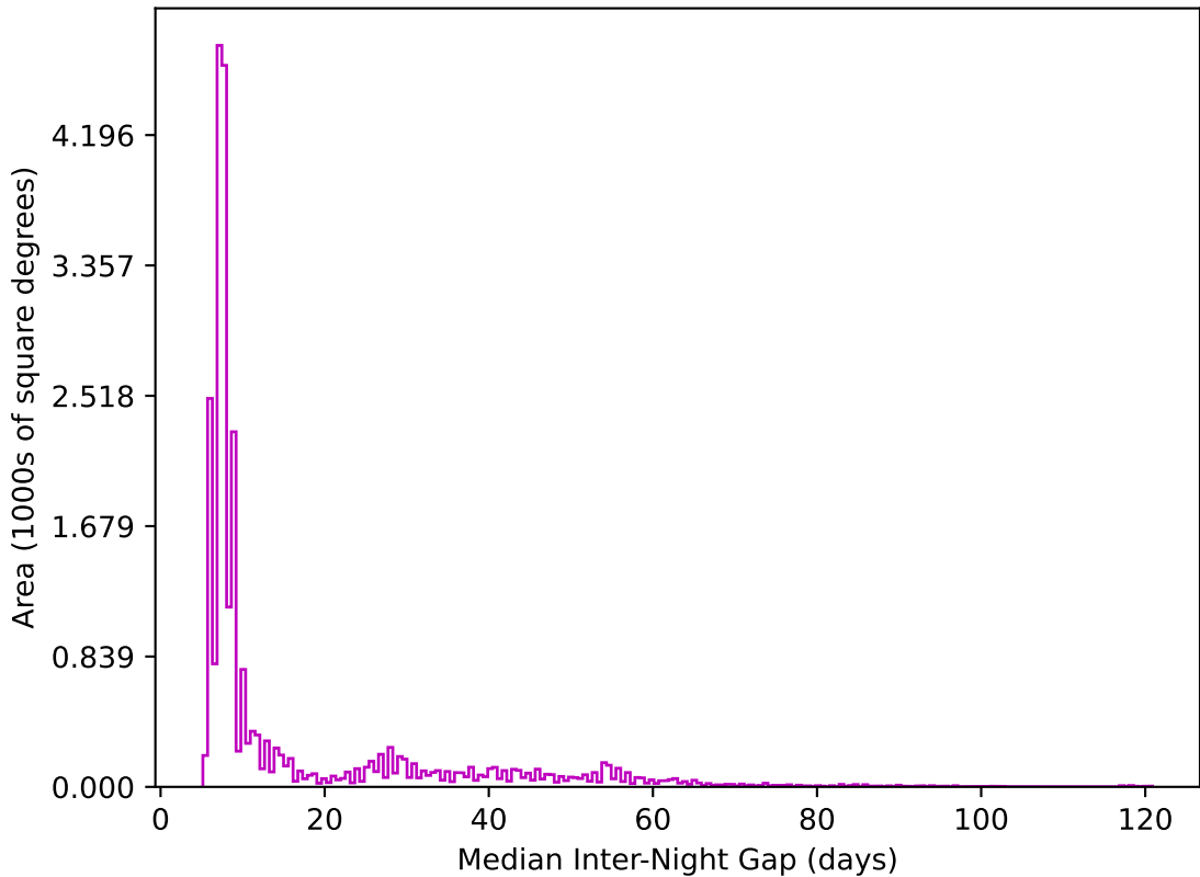
too_elab_r8_d2_giz_v3.4_10yrs All sky z band: Median Inter-Night Gap
