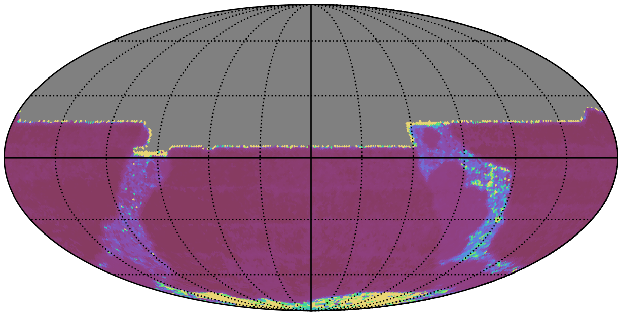
too_elab_r8_d2_giz_v3.4_10yrs All sky y band: Median Inter-Night Gap
