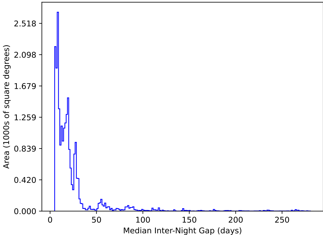
too_elab_r8_d2_giz_v3.4_10yrs All sky y band: Median Inter-Night Gap
