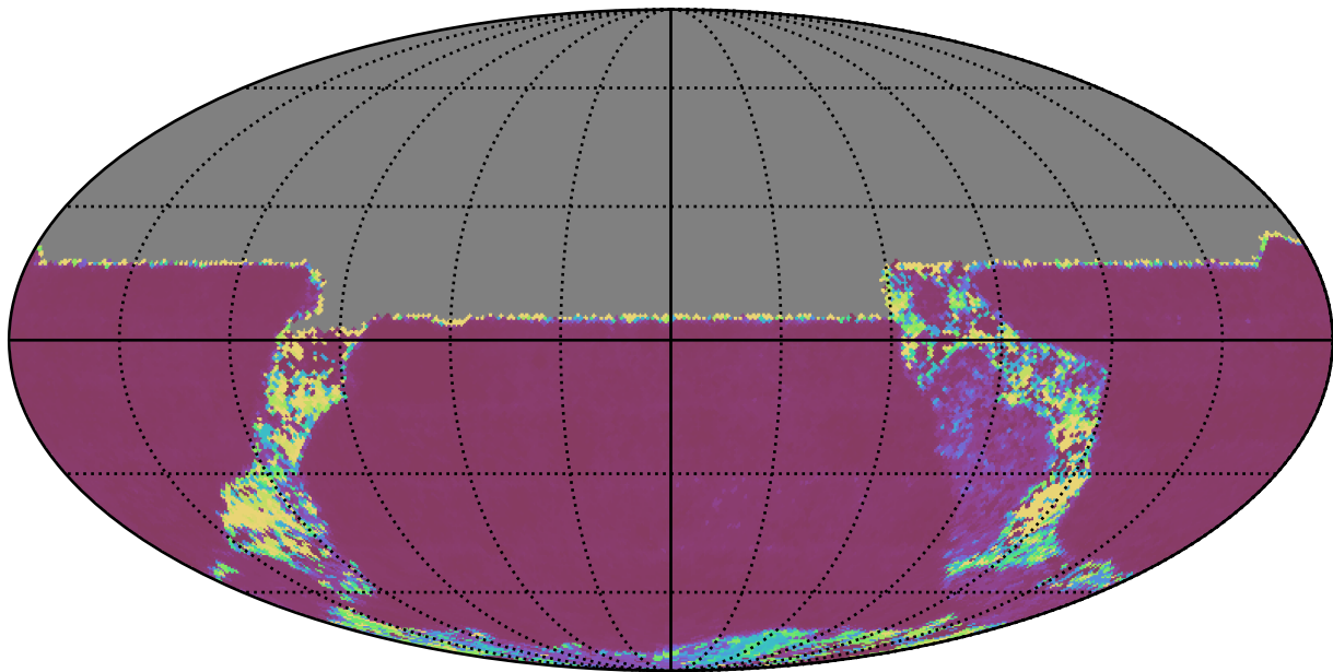
too_elab_r8_d2_giz_v3.4_10yrs All sky u band: Median Inter-Night Gap
