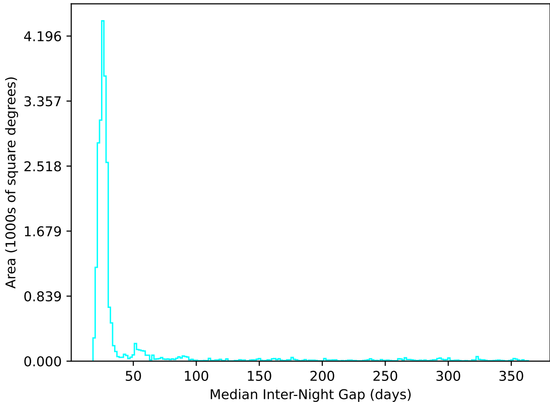
too_elab_r8_d2_giz_v3.4_10yrs All sky u band: Median Inter-Night Gap
