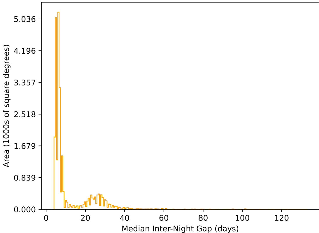
too_elab_r8_d2_giz_v3.4_10yrs All sky r band: Median Inter-Night Gap
