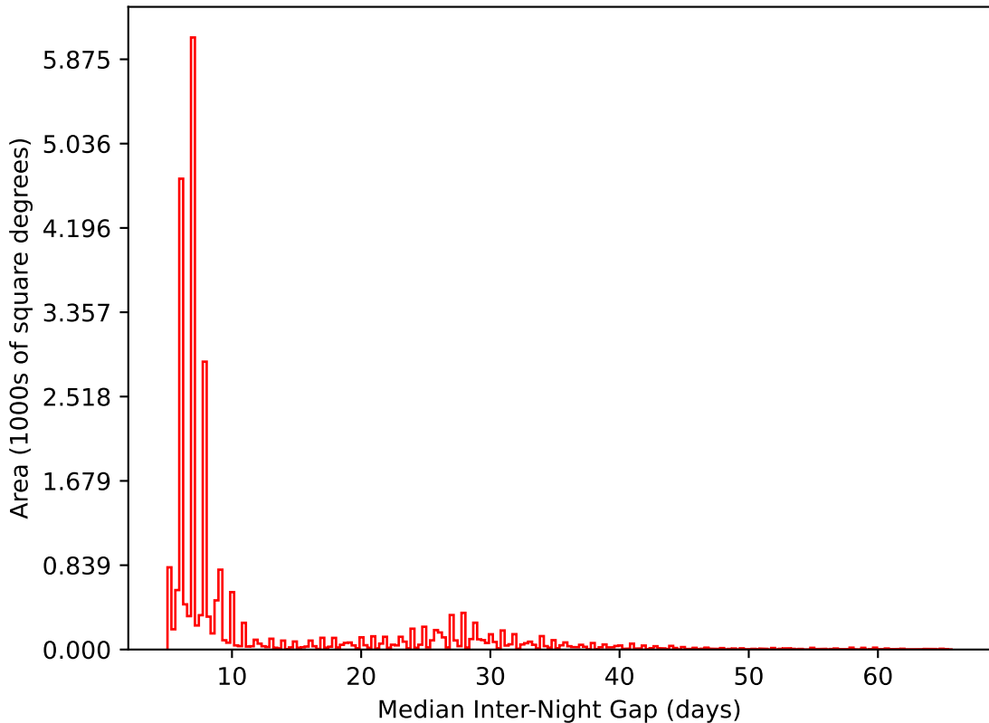
too_elab_r8_d2_giz_v3.4_10yrs All sky i band: Median Inter-Night Gap
