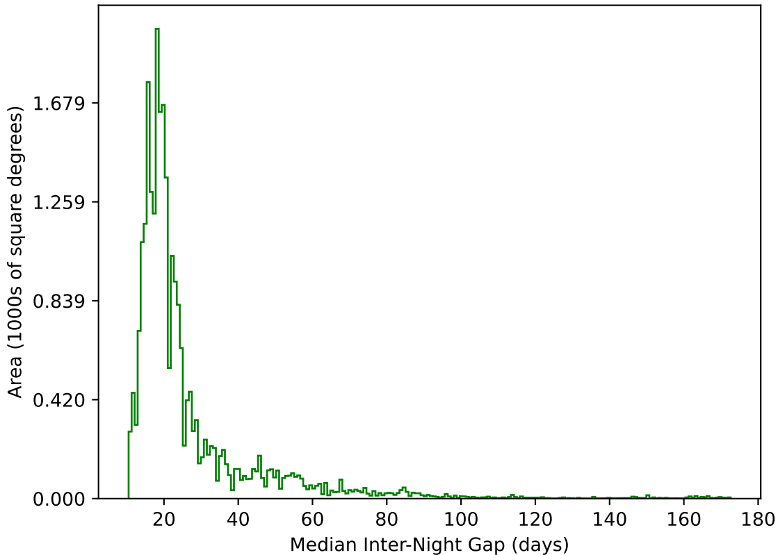
too_elab_r8_d2_giz_v3.4_10yrs All sky g band: Median Inter-Night Gap
