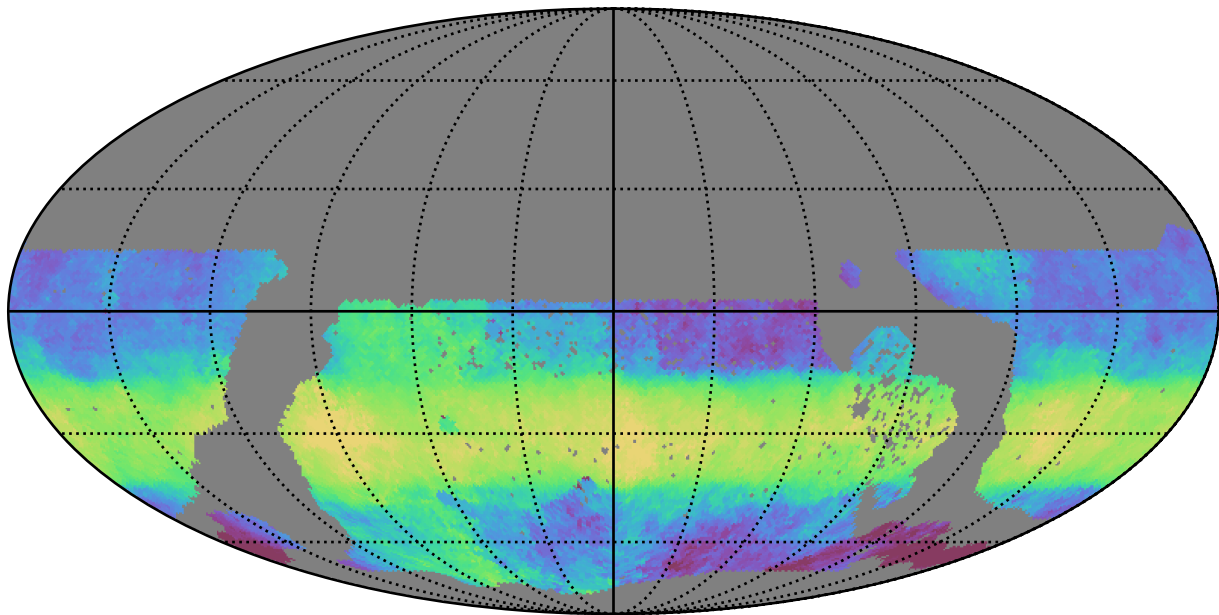
too_elab_r8_d2_giz_v3.4_10yrs WFD z band: Median HA
