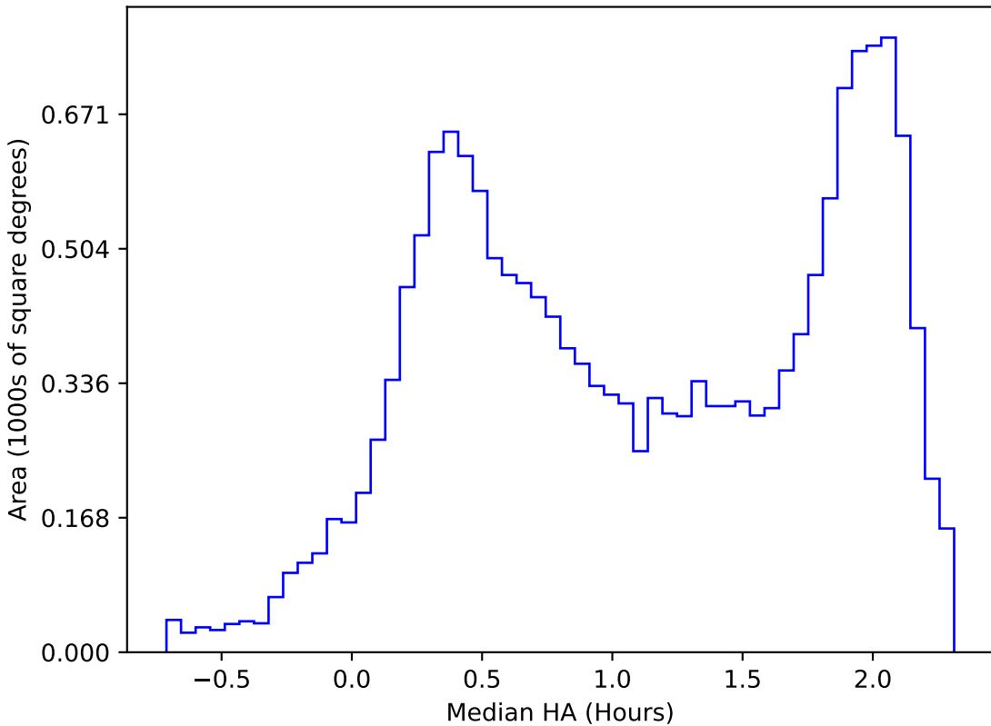
too_elab_r8_d2_giz_v3.4_10yrs WFD z band: Median HA
