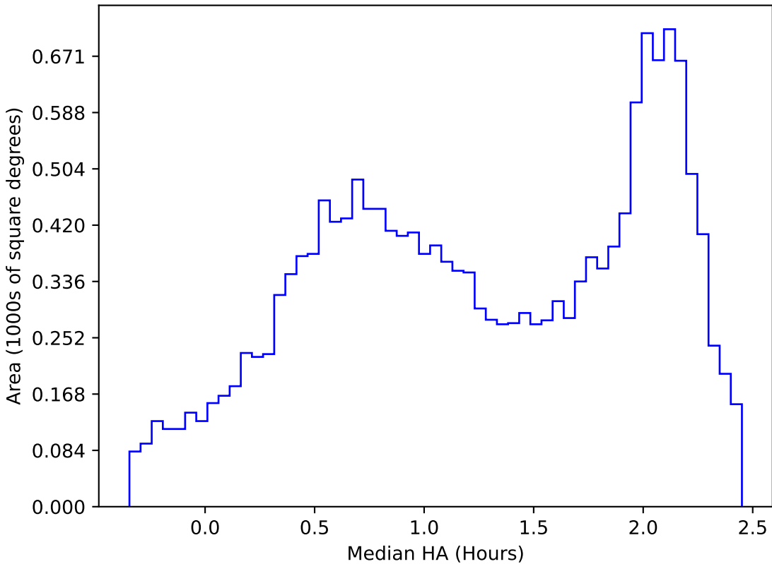
too_elab_r8_d2_giz_v3.4_10yrs WFD y band: Median HA
